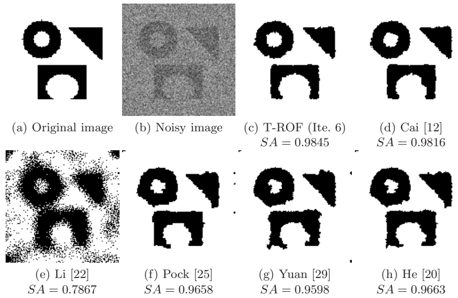
Fig. 1. Segmentation of two-class cartoon image ( 256 \times 256 ) with some missing pixel values.
