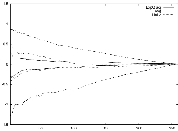
Figure 4: P-cone for range queries
