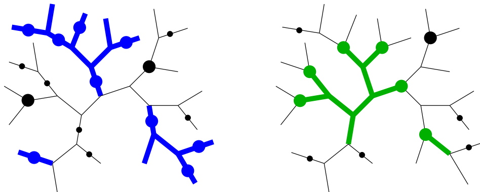
A Welschinger curve
