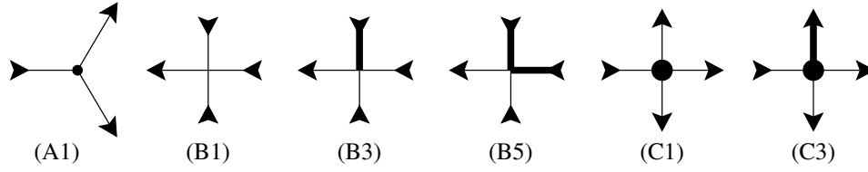
two vertices of type (1) – (6) merging
