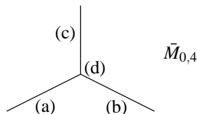
FIGURE 18. \bar{M}_{0,4} is again a rational tropical curve
