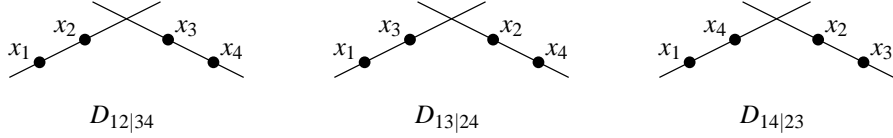
FIGURE 16. The three special points in \bar{M}_{0,4}
