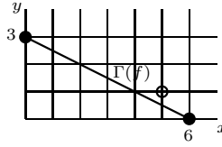
FIGURE 3. The Newton polygon of f = x^6 + y^3 + x^5y .
