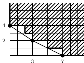
FIGURE 10. The Newton polygon of x^7 + x^3y^2 + y^4 for \text{char}(K) \neq 2, 3, 7 .
